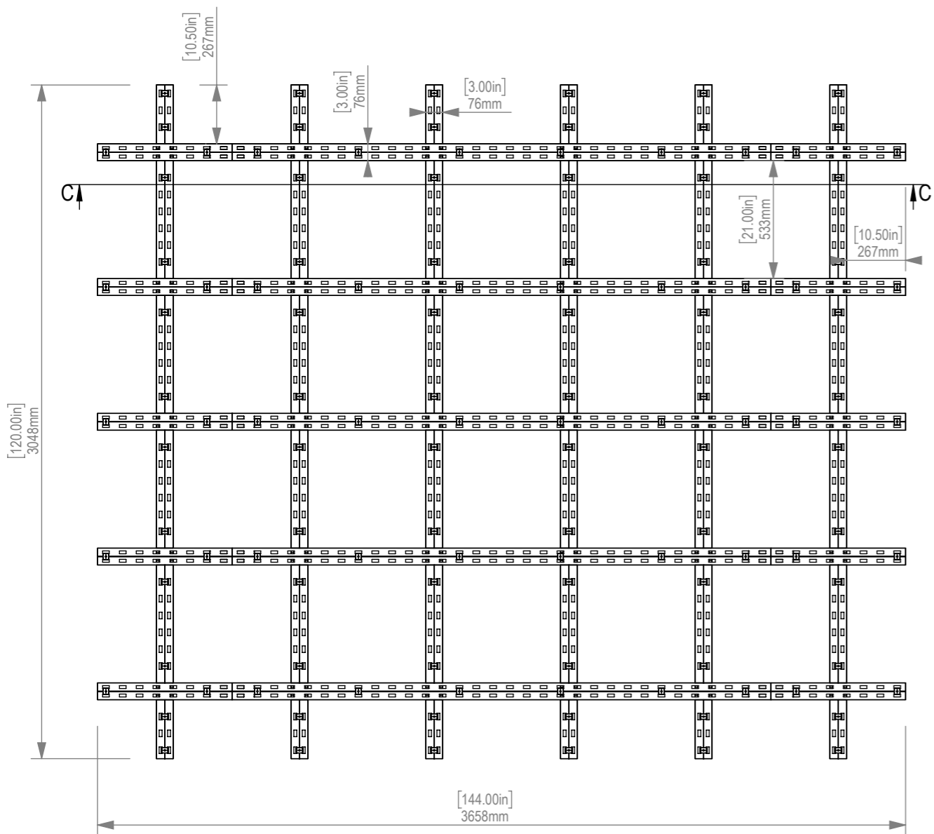
TOP VIEW
