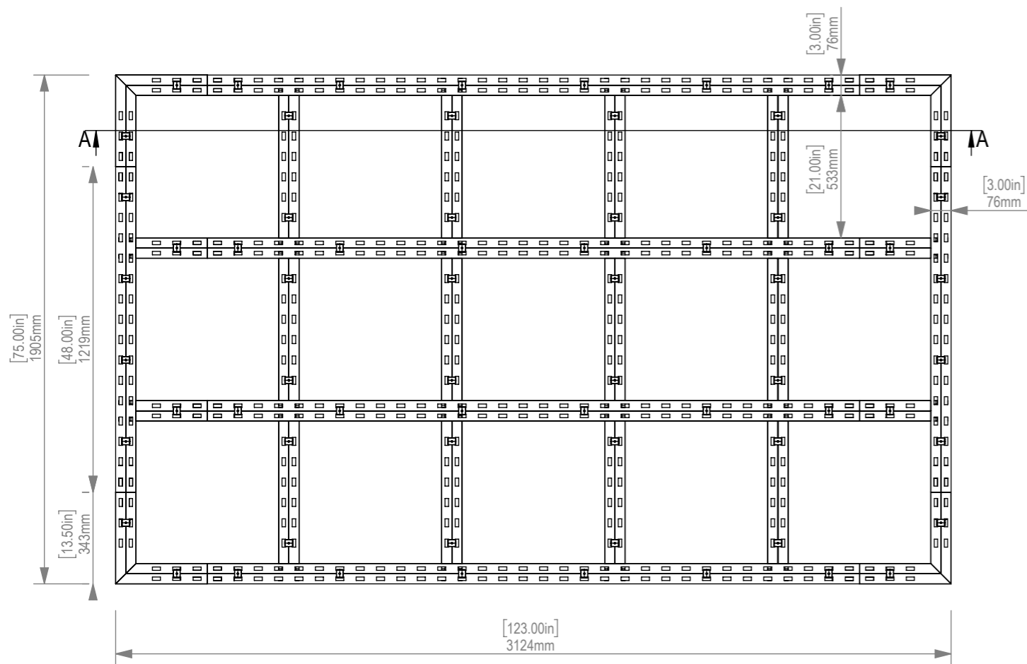
TOP VIEW
